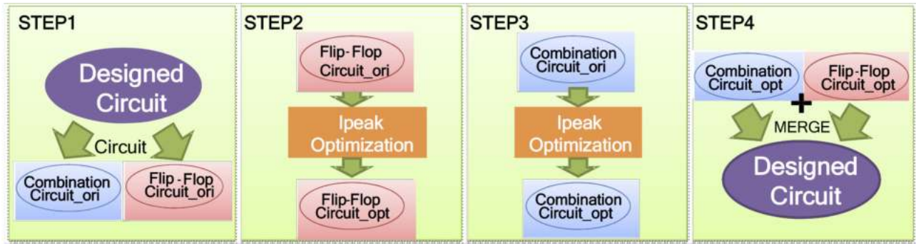
Figure 10. The sequential circuit processing flow in the proposed IPR.
