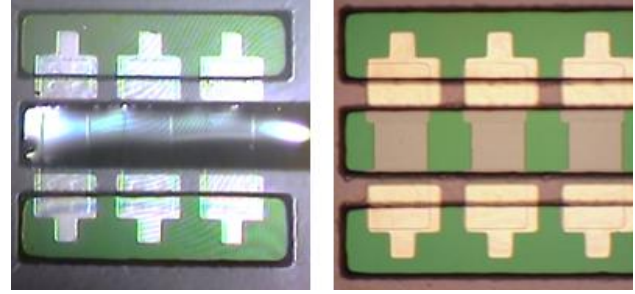
(A) (B) Figure 3. Fabricated ISFETs with (a) and without (b) the solution in the gate region.
